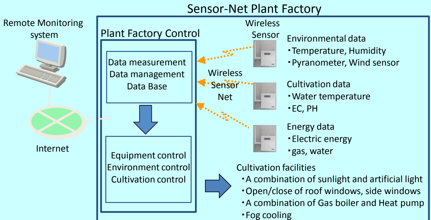
Fig. 1. Sensor-net Plant Factory System
